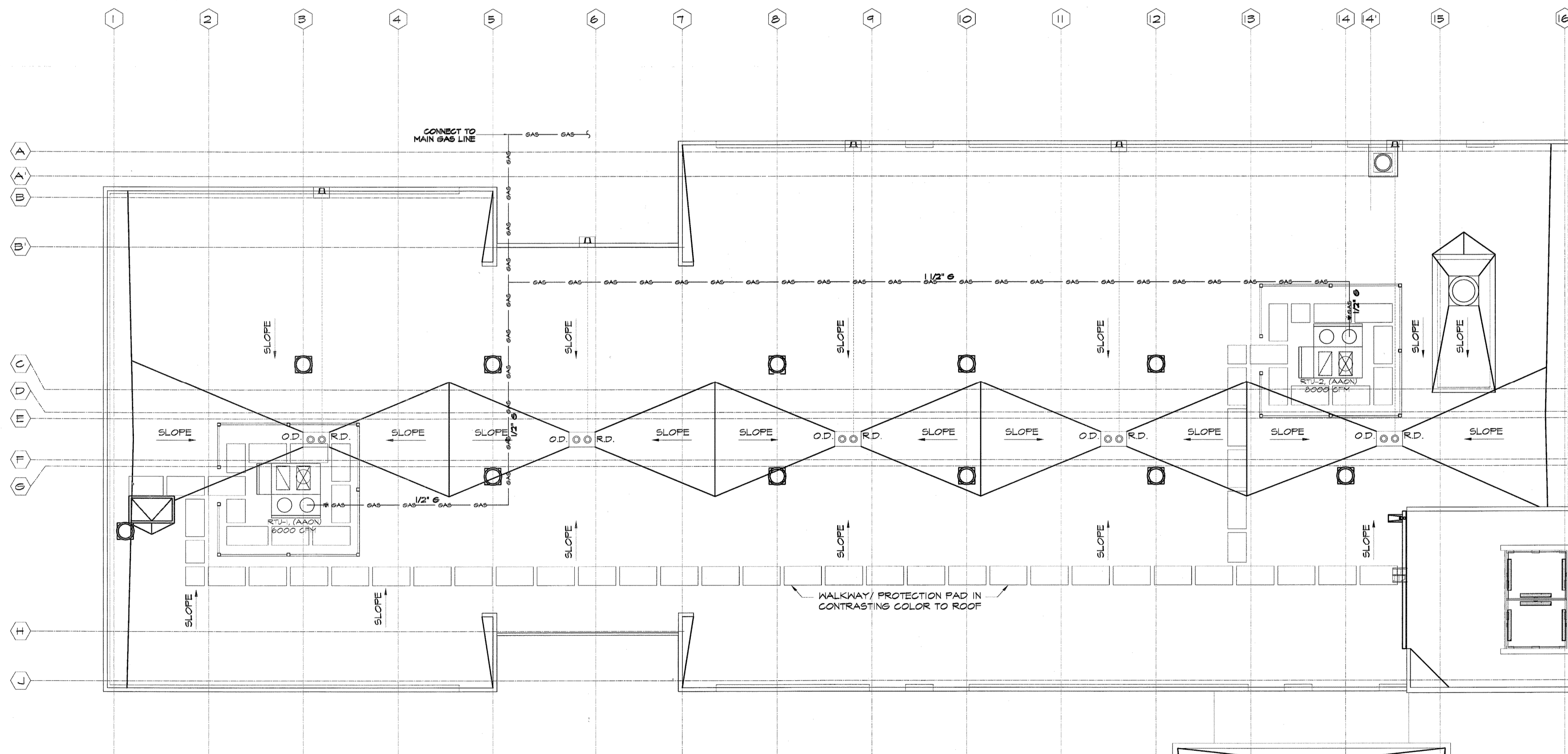
O2 ROOF TOP UNIT GAS LAYOUT PLAN SCALE: 1/8" = 1'-0"
